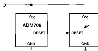
Typical Operating Circuit
