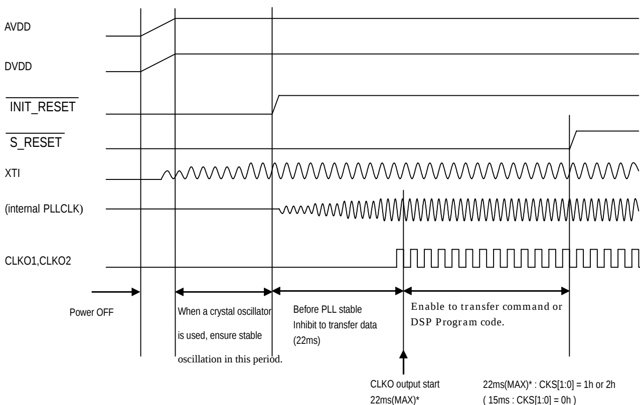
Fig. Power supply startup sequence
