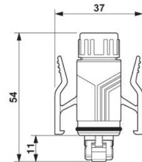
RJ45-plug connector, IP67
