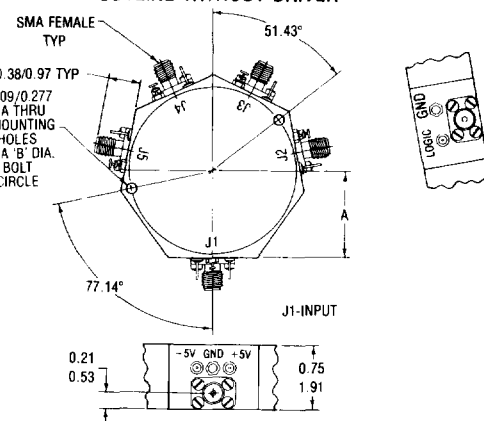
CONFIGURATION S OUTLINE WITHOUT DRIVER
