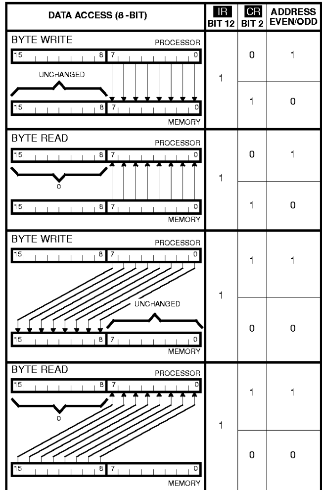
FIGURE 19. MEMORY ACCESS (BYTE)
