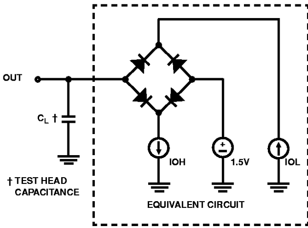
FIGURE 20. TEST CIRCUIT
