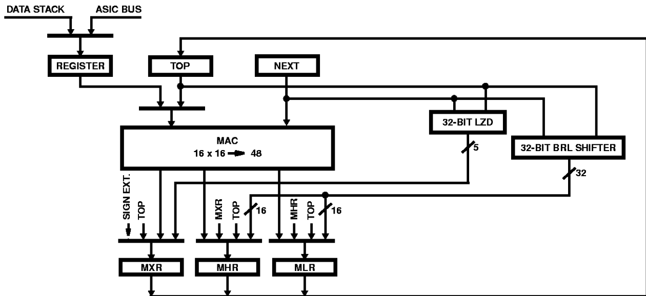
FIGURE 17. HS-RTX2010RH FLOATING POINT/DSP LOGIC
