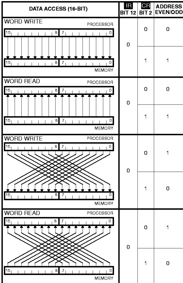
FIGURE 18. MEMORY ACCESS (WORD)
