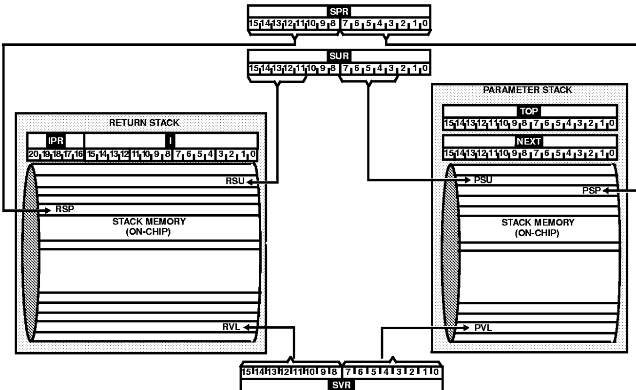
FIGURE 14. DUAL STACK ARCHITECTURE
