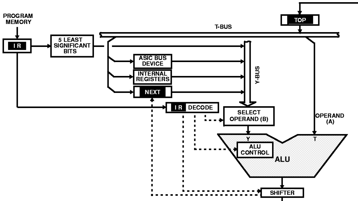
FIGURE 16. ALU OPERATIONS-CONTROL PATHS AND DATA FLOW
