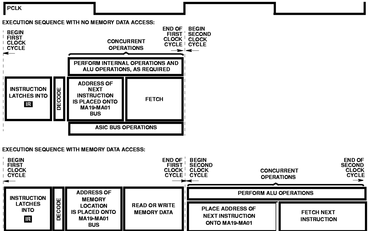
FIGURE 2. INSTRUCTION EXECUTION SEQUENCE
