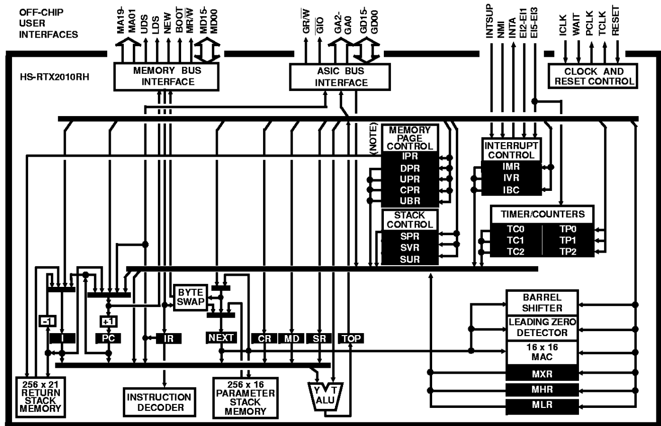
FIGURE 1. HS-RTX2010RH FUNCTIONAL BLOCK DIAGRAM
