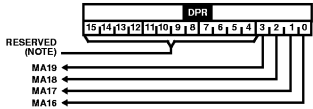
FIGURE 12. DPR BIT ASSIGNMENTS
