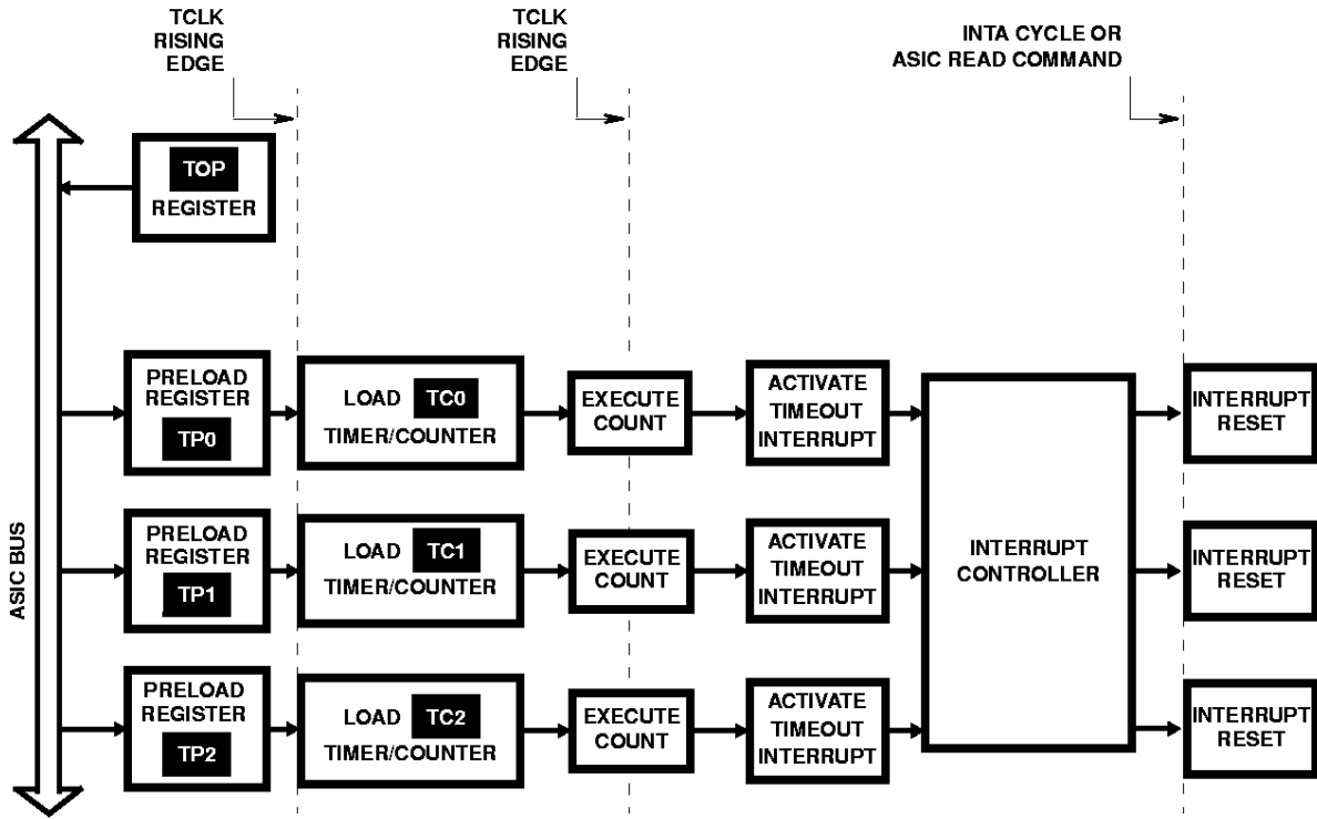
FIGURE 15. HS-RTX2010RH TIMER/COUNTER OPERATION
