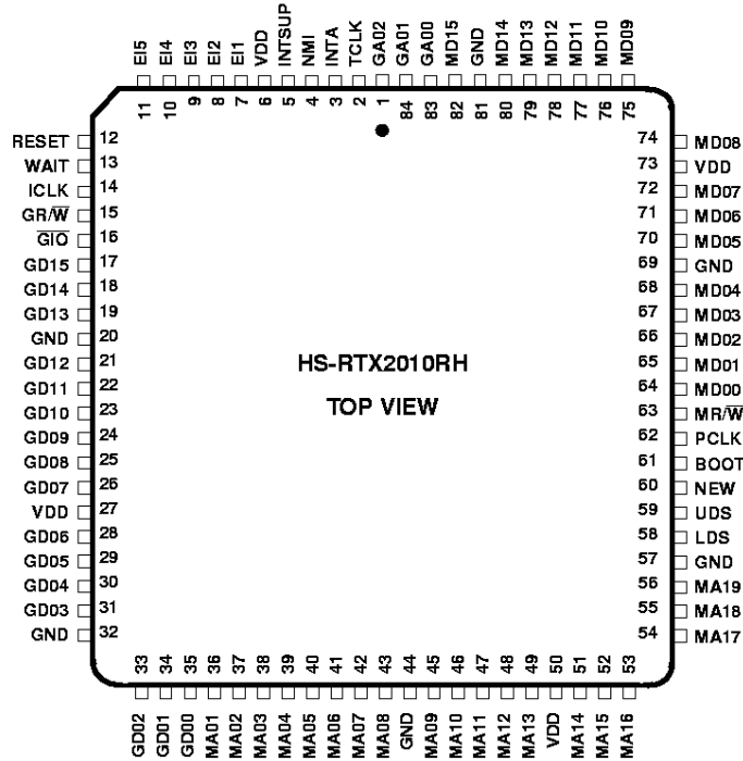
HS9-RTX2010RH (LEAD LENGTH NOT TO SCALE) SEE HARRIS OUTLINE R84.A
