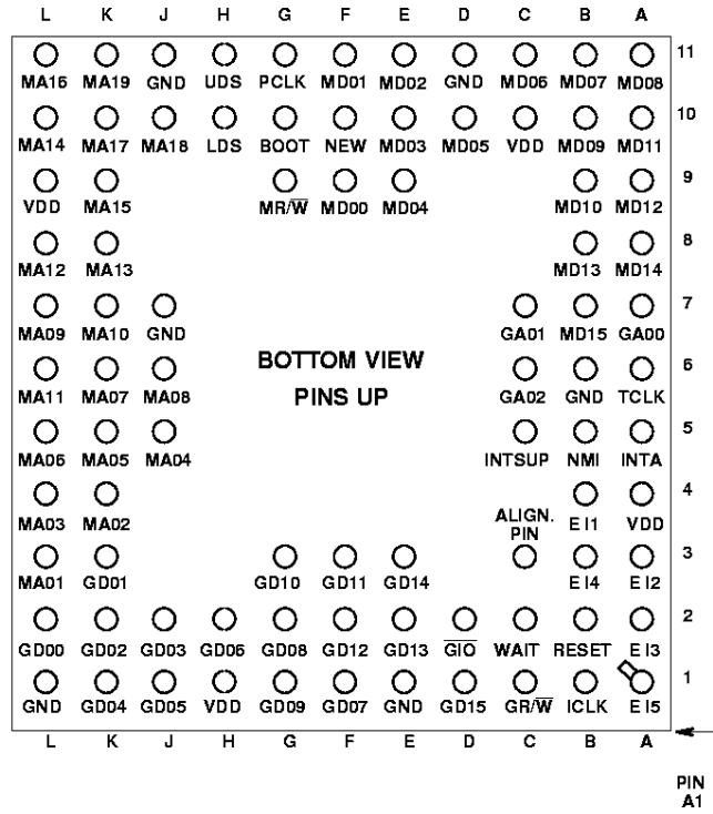
HS9-RTX2010RH (LEAD LENGTH NOT TO SCALE) SEE HARRIS OUTLINE R84.A
