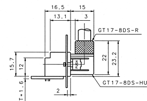
Mating Diagram
