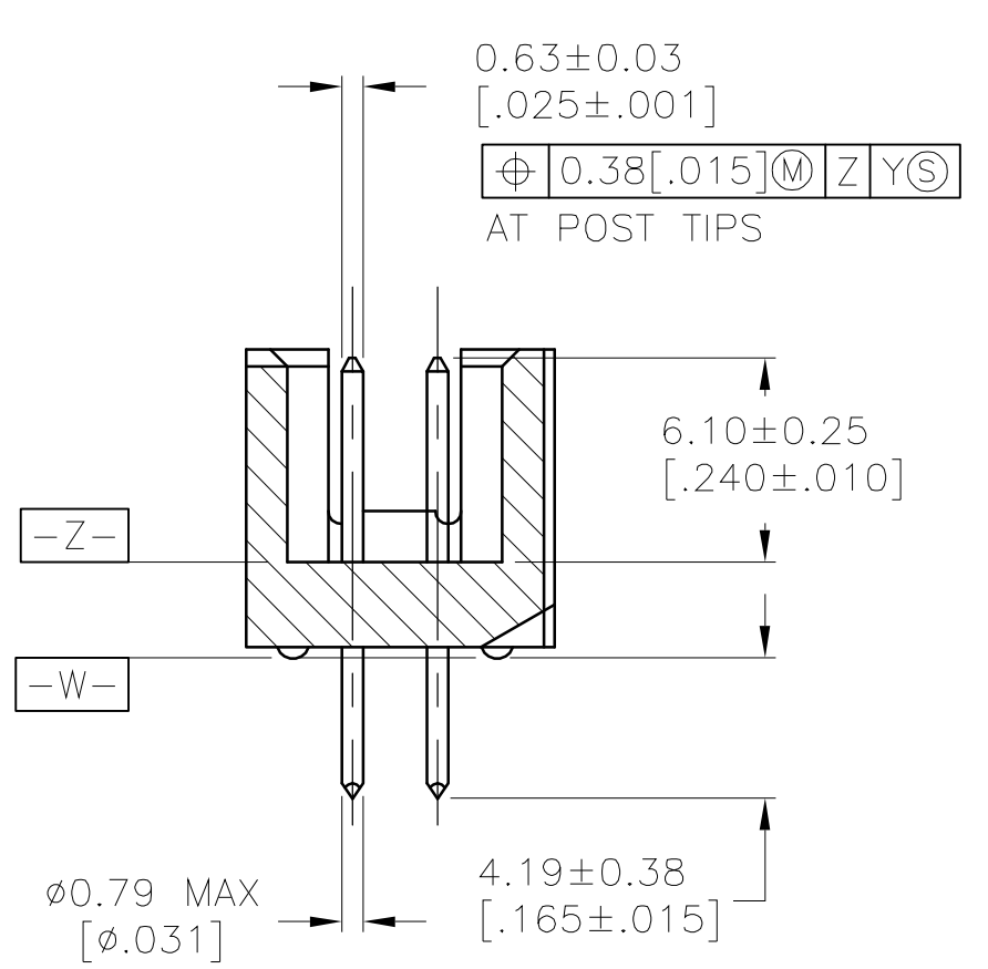
SECTION U-U
