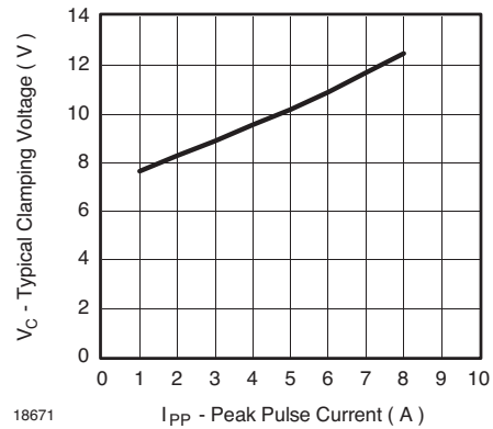
Figure 6. Typical Clamping Voltage vs. Peak Pulse Current
