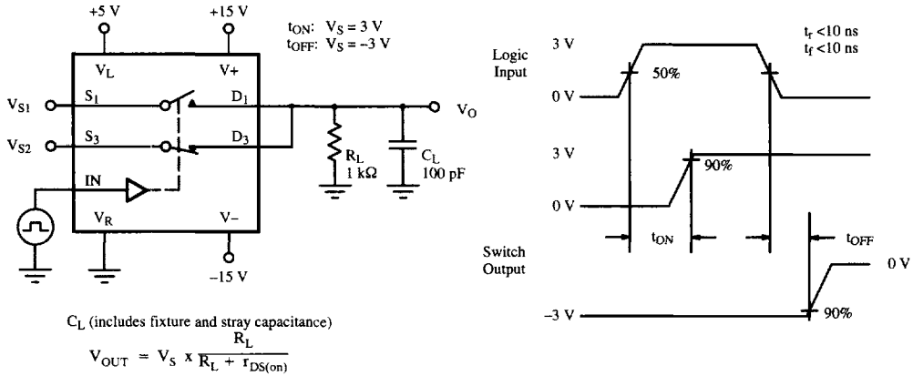
Figure 2. Switching Time
