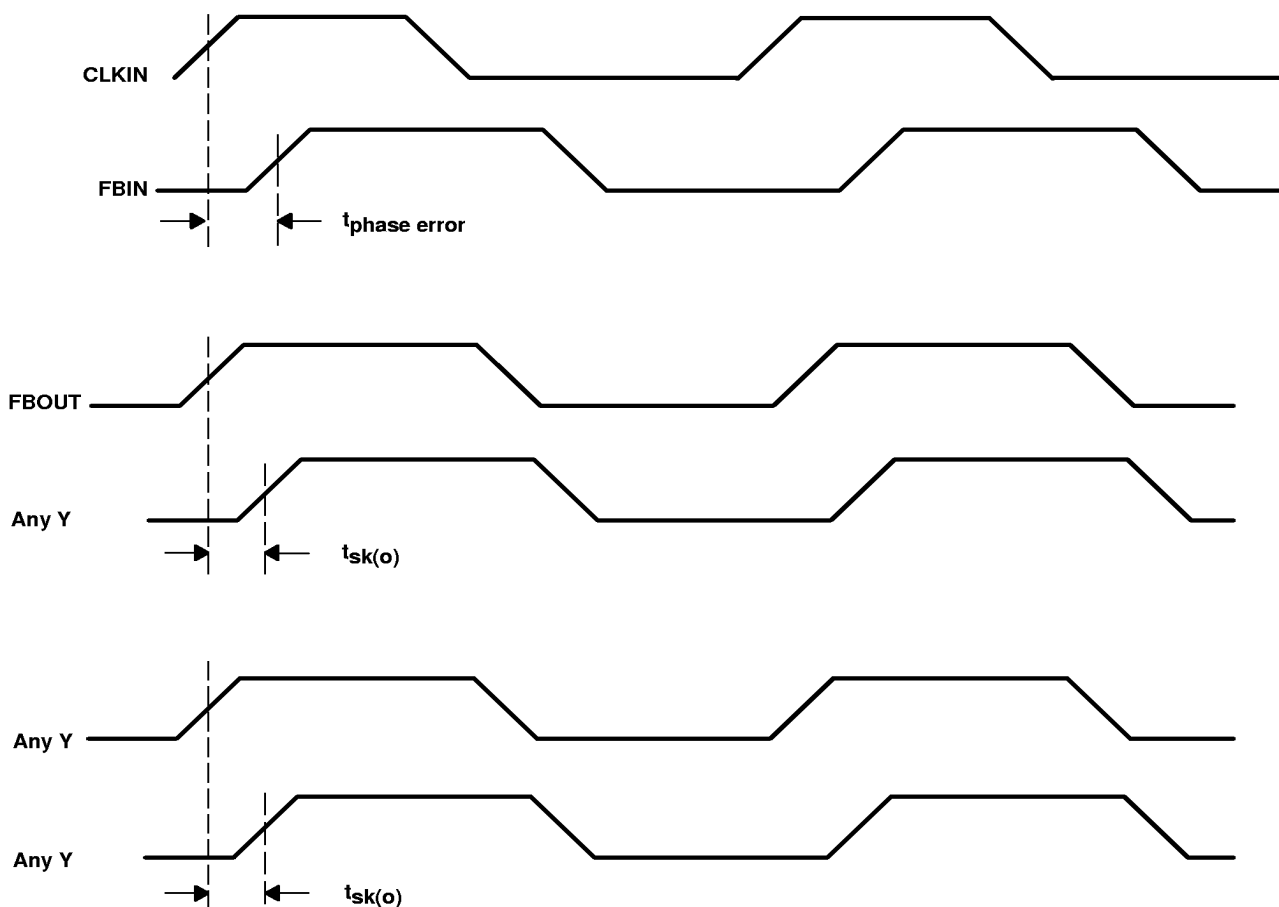
Figure 2. Phase Error and Skew Calculations
