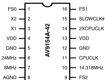
16-Pin PDIP or SOIC AV9154A-42
