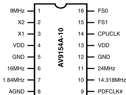
16-Pin PDIP or SOIC AV9154A-10
