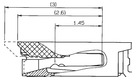
SECT X-X
