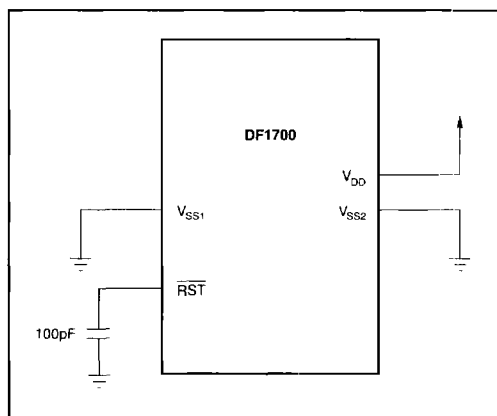
FIGURE 4. System Reset Circuit.
