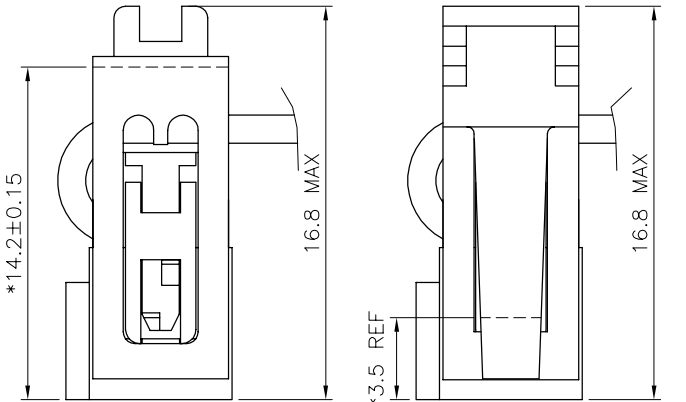
WITH STANDARD STRAIN RELIEF WITH LATCHING STRAIN RELIEF
