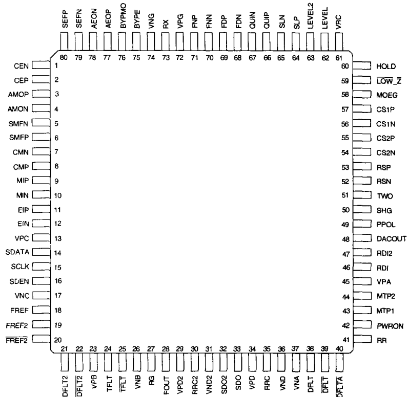
80-Lead TQFP
