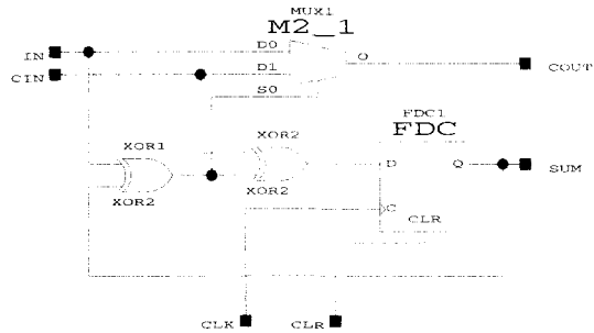
Figure 20: Accumulator Schematic
