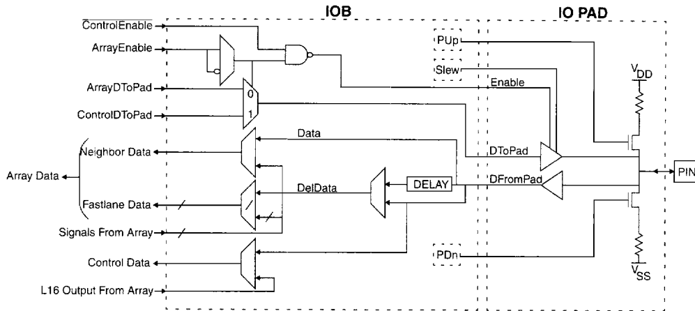
Figure 15: Input/Output Architecture
