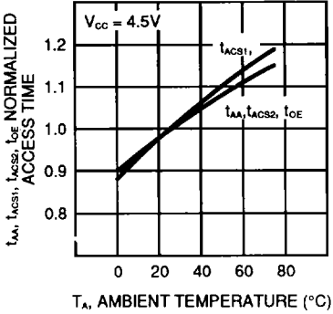
Fig. 4 – NORMALIZED ACCESS TIME vs. AMBIENT TEMPERATURE
