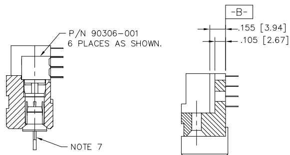
SECTION P-P SECTION W-W
