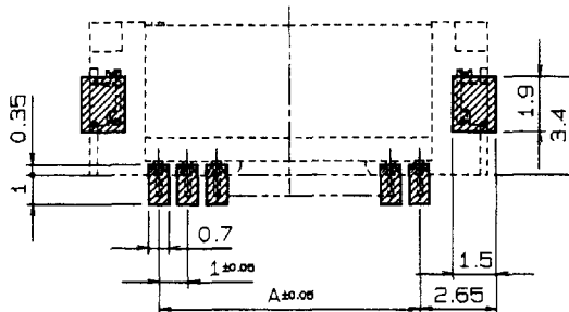
MOUNTING LAYOUT
