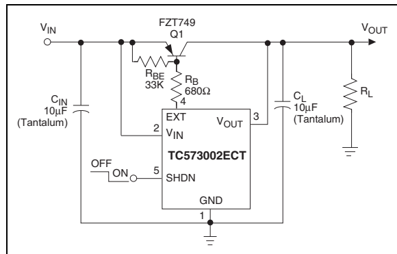
FIGURE 3-1: TEST CIRCUIT
