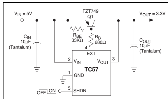
FIGURE 3-2: 3.3V, 1A REGULATOR USING 5V SUPPLY INPUT
