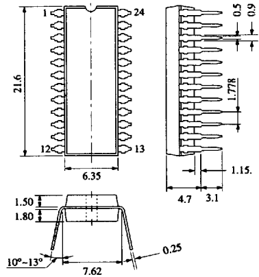
24-Lead Shrink DIP Plastic Package (24-SDIP)
