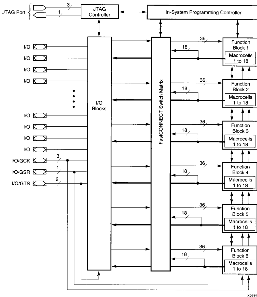
Figure 2: XC95108 Architecture
