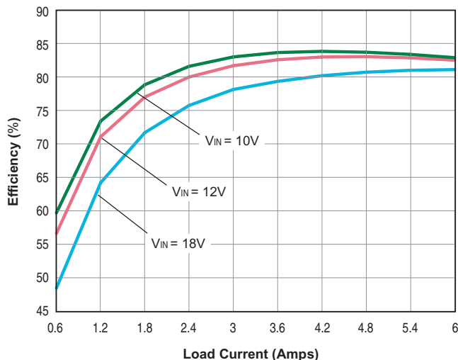
UWR-1.8/6000-D12A Efficiency vs. Line and Load
