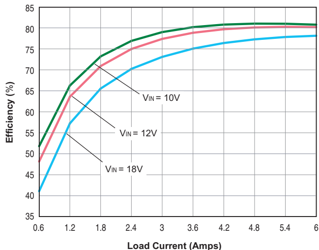
UWR-1.5/6000-D12A Efficiency vs. Line and Load
