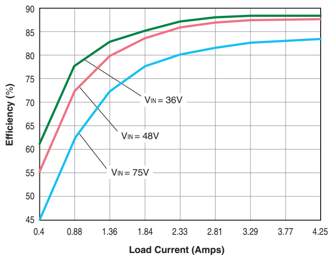
UWR-3.3/4500-D48ANT Efficiency vs. Line and Load
