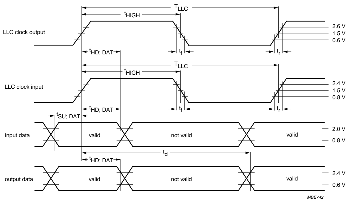
Fig.7 Clock data timing.
