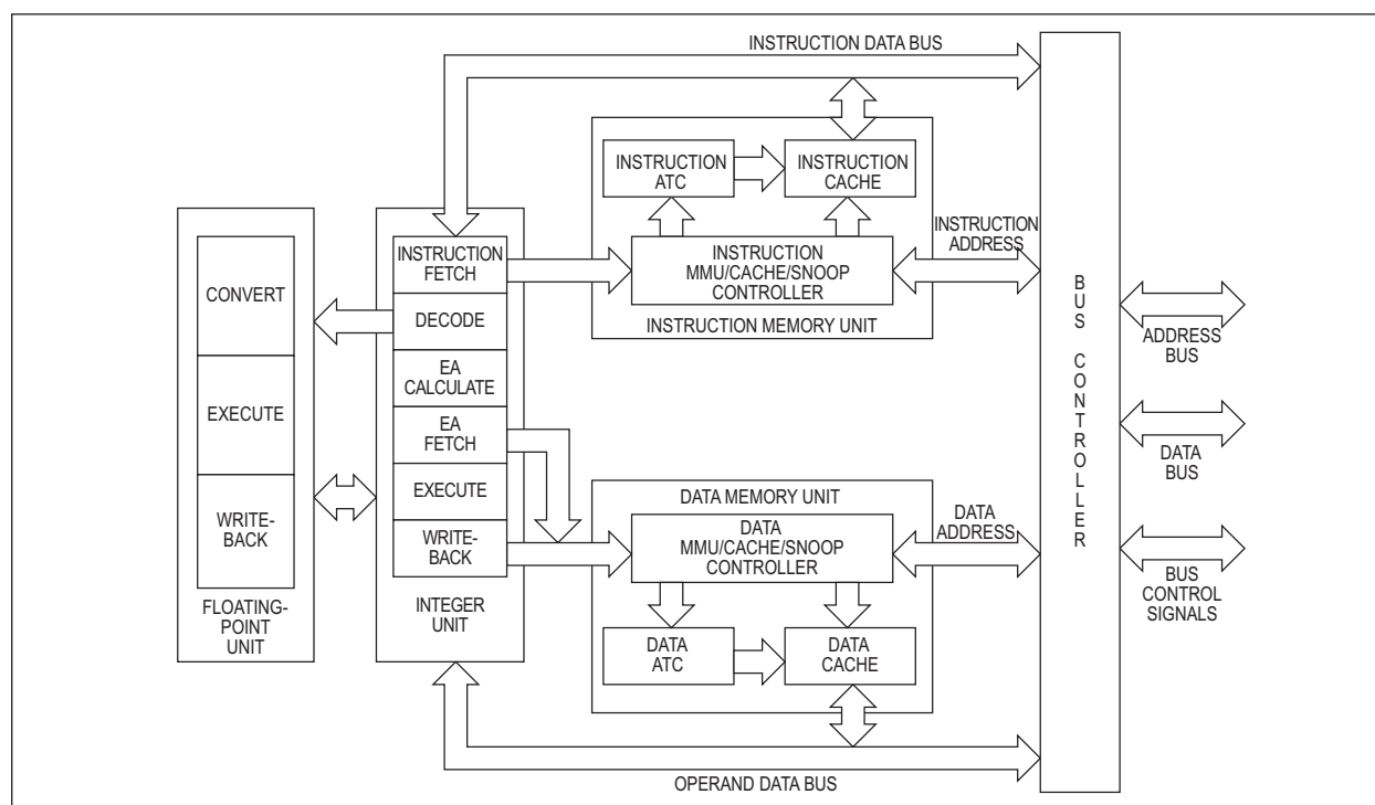
FIGURE 1 – BLOCK DIAGRAM
