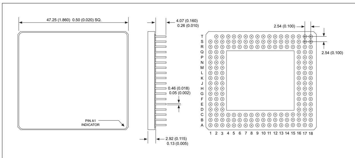
FIGURE 12 179 PIN GRID ARRAY, PGA (P4)
