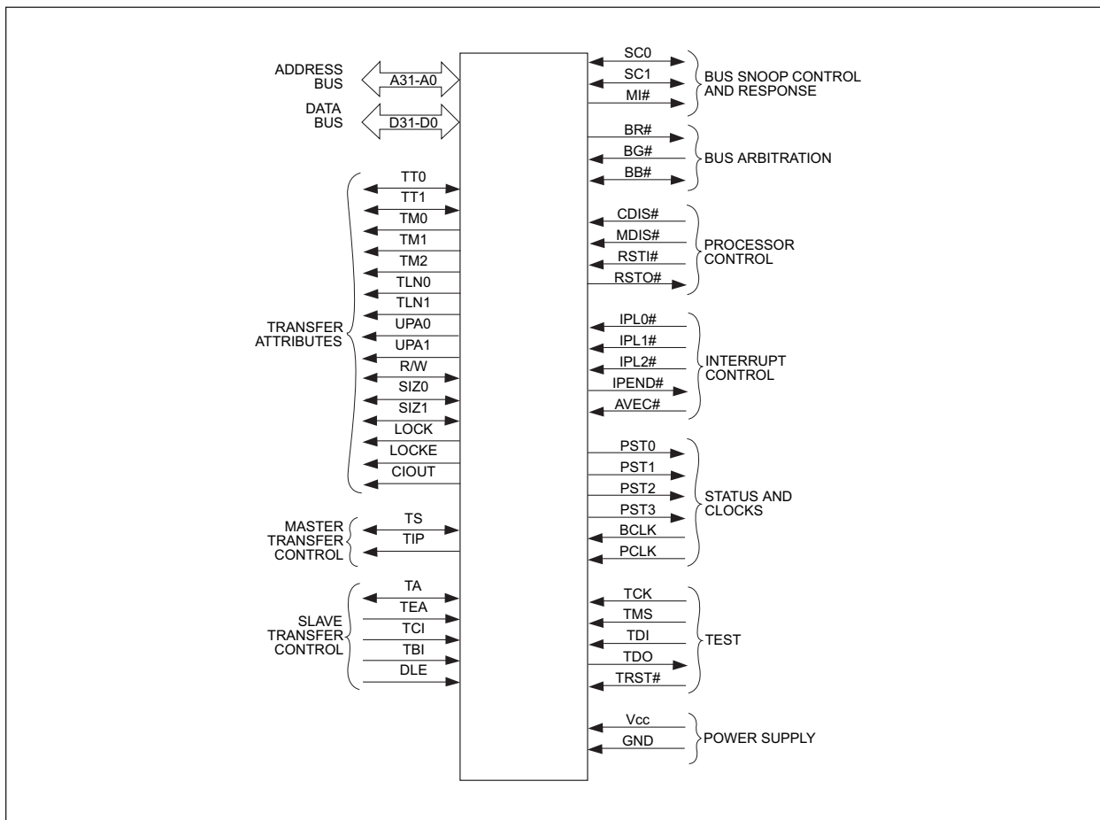
FIGURE 4 – FUNCTIONAL SIGNAL GROUPS
