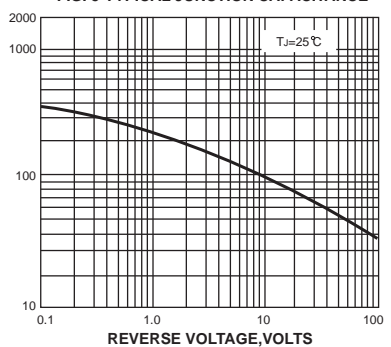
FIG. 5-TYPICAL JUNCTION CAPACITANCE
