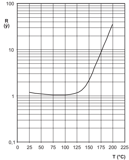
TYPICAL RESISTANCE/TEMPERATURE CHARACTERISTIC for 2322 662 51224.
