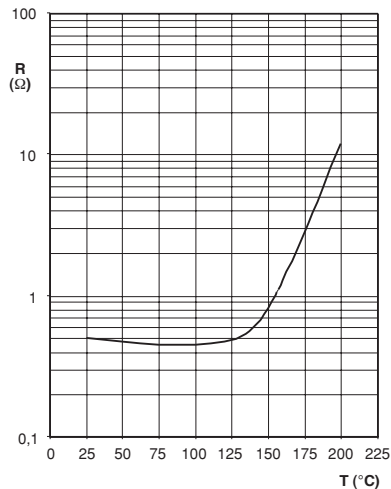
TYPICAL RESISTANCE/TEMPERATURE CHARACTERISTIC for 2322 662 51224.
