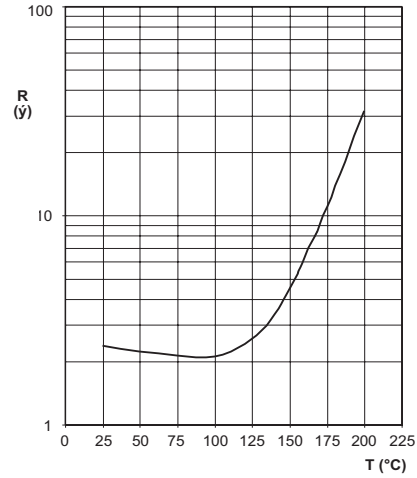
TYPICAL RESISTANCE/TEMPERATURE CHARACTERISTIC for 2322 661 57014.
