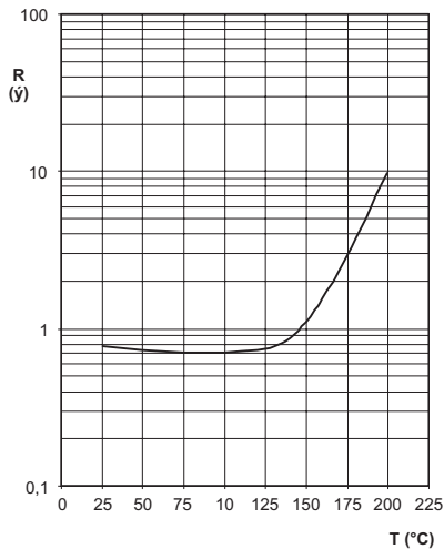
TYPICAL RESISTANCE/TEMPERATURE CHARACTERISTIC for 2322 661 59014.
