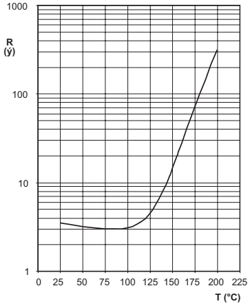
TYPICAL RESISTANCE/TEMPERATURE CHARACTERISTIC for 2322 660 54714.
