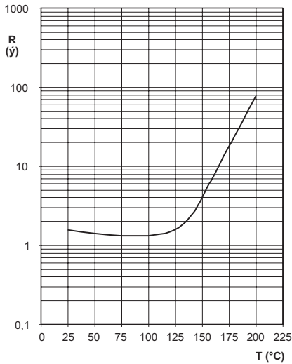
TYPICAL RESISTANCE/TEMPERATURE CHARACTERISTIC for 2322 661 59014.
