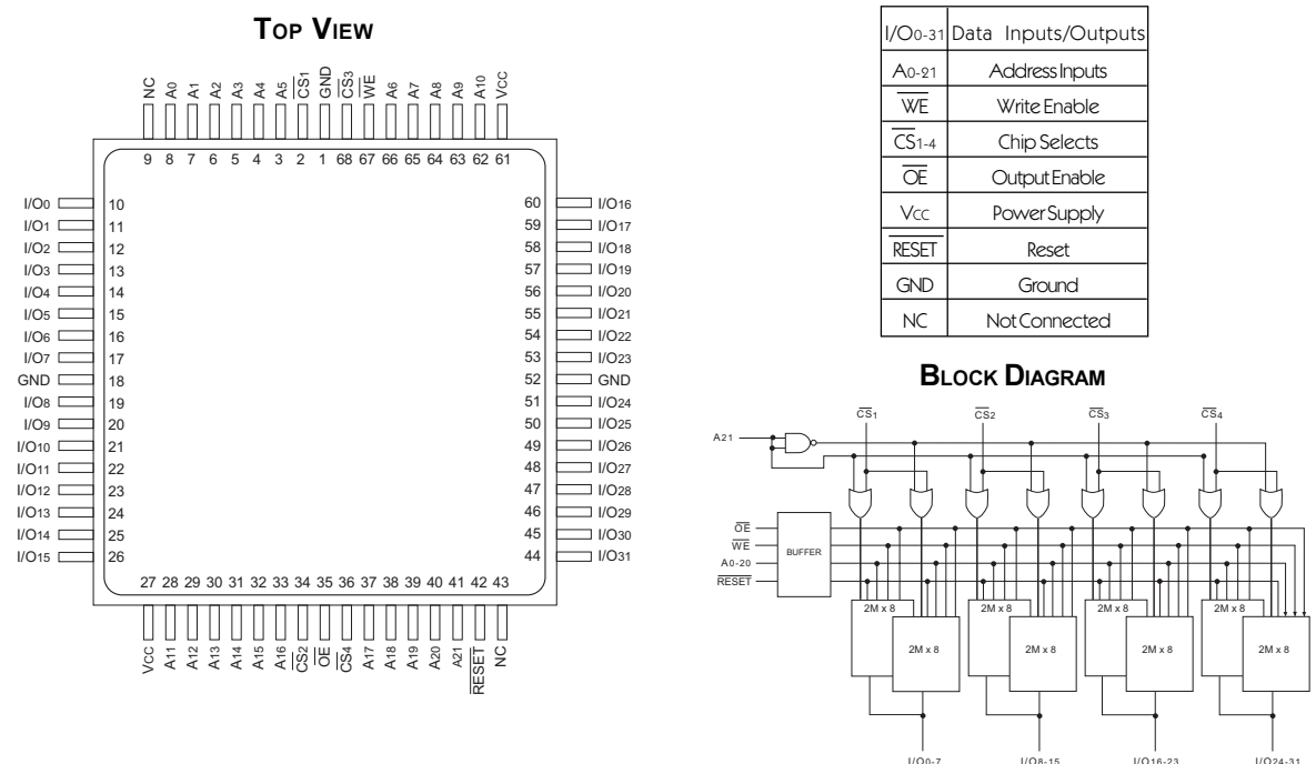
FIG. 2 PIN CONFIGURATION FOR WF4M32-XG4TX5
