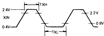
External Clock Input (8.0 MHz Max.)
