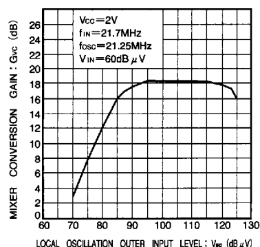
Fig. 6 Mixer conversion gain vs. Pin 2 OSC injection level characteristic
