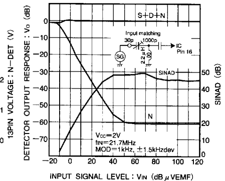
Fig. 15 Detector output response, SINAD vs. input signal level characteristic
