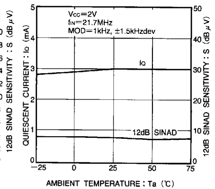
Fig. 9 Quiescent current, 12 dB SINAD sensitivity vs. ambient temperature characteristic
