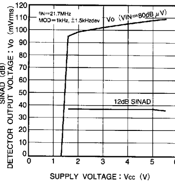
Fig. 8 Detector output voltage, 12 dB SINAD sensitivity vs. power supply voltage characteristic
