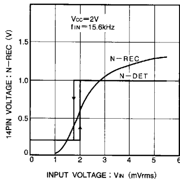
Fig. 14 Pin 13 voltage, Pin 14 voltage vs. noise amplifier input voltage characteristic
