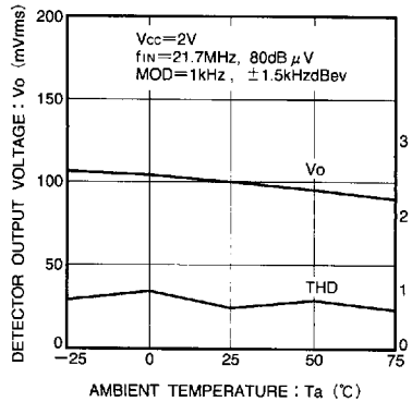
Fig. 10 Detector output level, THD vs. ambient temperature characteristic
