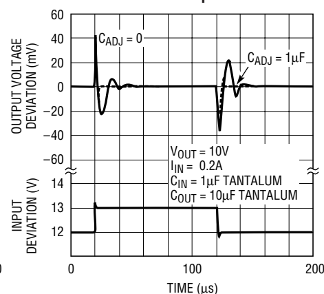
LT1085 Line Transient Response
