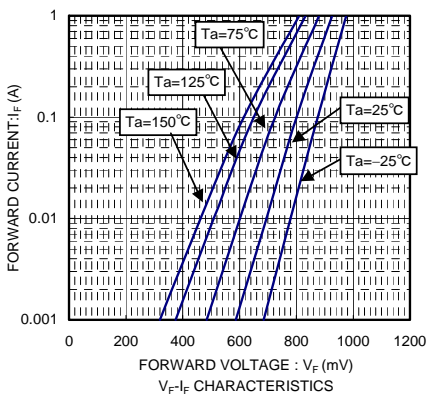
V_F - I_F CHARACTERISTICS
