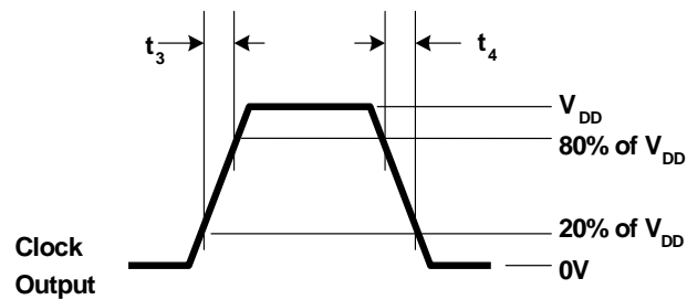
Figure 3. ER = (0.6 \times V_{DD}) / t_3 , EF = (0.6 \times V_{DD}) / t_4
