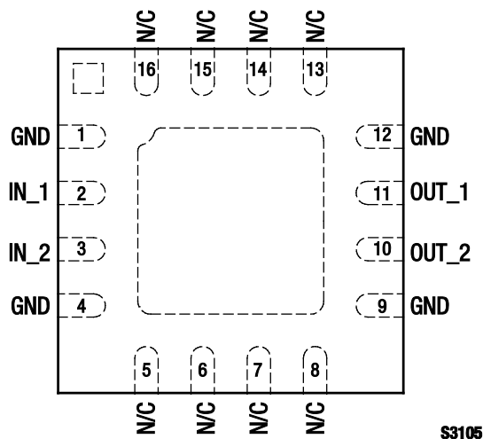
Figure 2. SKY12213-478LF Pinout – 16-Pin QFN (Top View)
