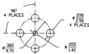
Recommended PCB Hole Configuration
