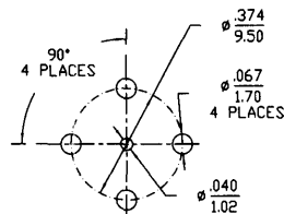
Recommended PCB Hole Configuration
