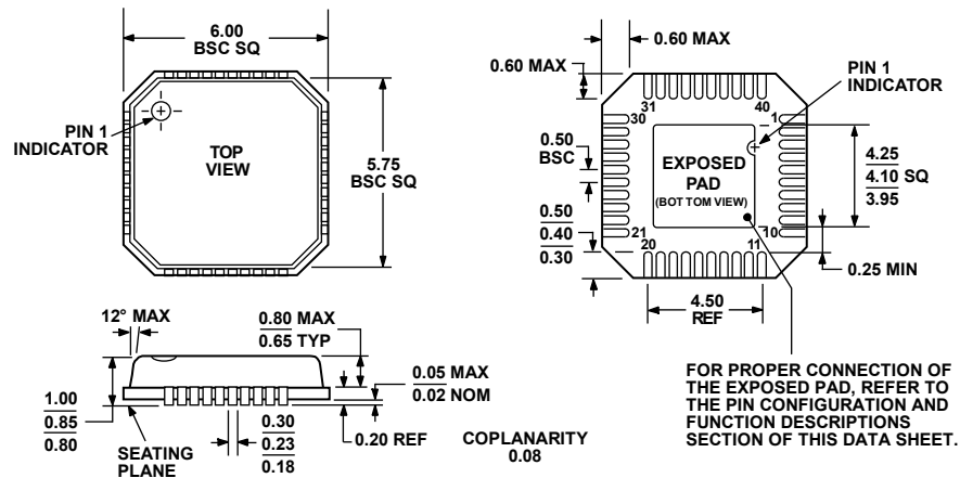
COMPLIANT TO JEDEC STANDARDS MO-220-VJJD-2 Figure 54. 40-Lead Lead Frame Chip Scale Package [LFCSP_VQ] 6 mm x 6 mm Body, Very Thin Quad (CP-40-1) Dimensions shown in millimeters
