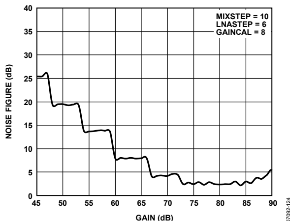
Figure 27. RXLBRF, Receiver Noise Figure vs. Gain, UMTS Band V, Rx Frequency = 836 MHz
