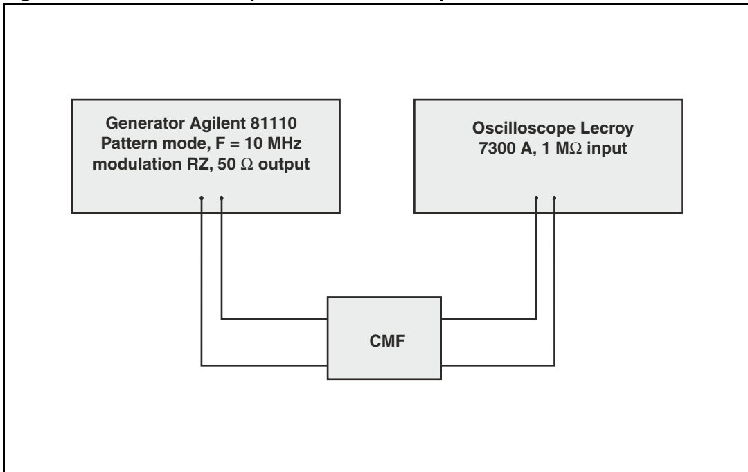
Figure 9. MIPI D-PHY low power mode test setup
