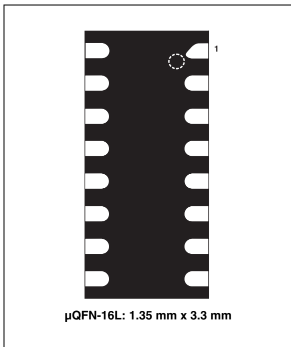
Figure 1. Pin configuration (top view)
