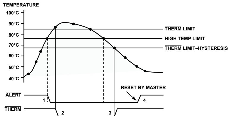
Figure 84. \overline{\text{THERM}} Behavior
