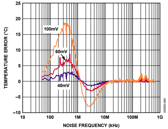
Figure 18. Remote Temperature Error vs. Common-Mode Noise Frequency
