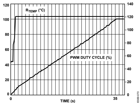
Figure 81. Enhanced Acoustics Mode with Ramp Rate = 1
