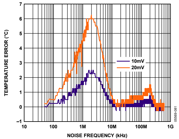
Figure 19. Remote Temperature Error vs. Differential-Mode Noise Frequency
