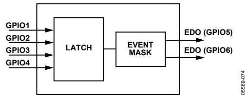
Figure 85. EDO Circuit
