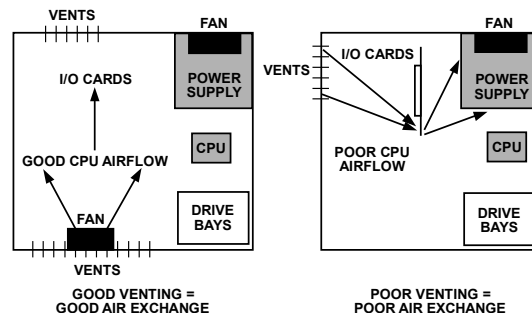
Figure 66. Chassis Airflow Issues
