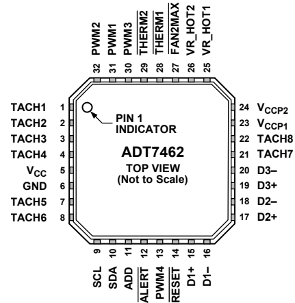
Figure 5. Configuration Option 2
