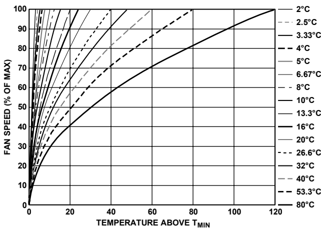
Figure 61. T_{RANGE} VS. Actual Fan Speed Profile
