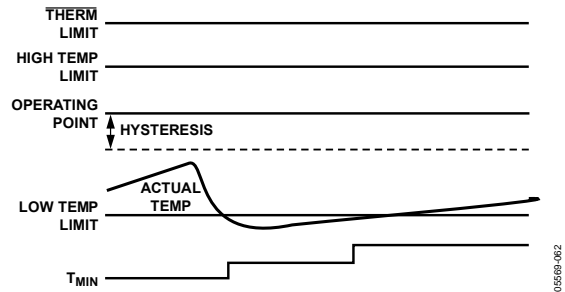
Figure 73. Increasing T MIN for Quieter Operation
