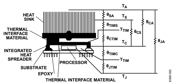
Figure 67. Thermal Model
