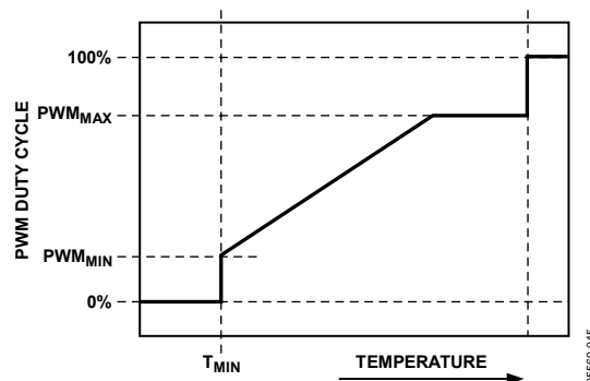
Figure 57. PWM MAX Determines Maximum PWM Duty Cycle Below the T THERM Temperature Limit
