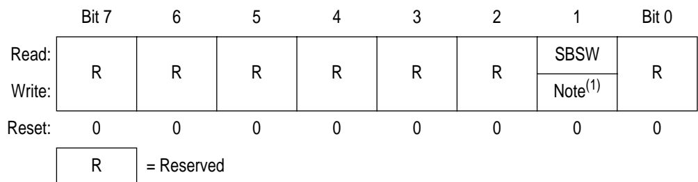
Figure 8-17. SIM Break Status Register (SBSR)
