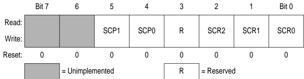
Figure 15-16. SCI Baud Rate Register (SCBR)
