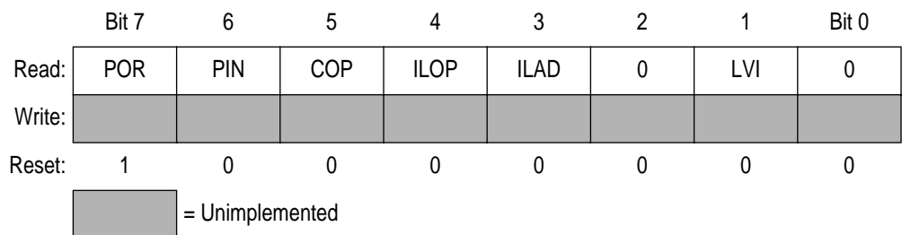
Figure 8-18. SIM Reset Status Register (SRSR)
