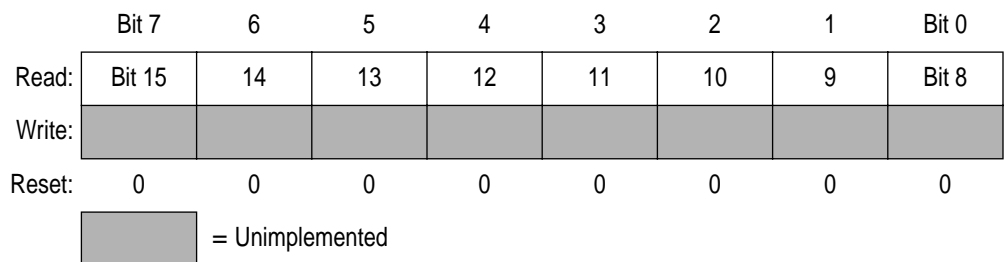
Figure 12-5. TIMB Counter Register High (TBCNTH)
