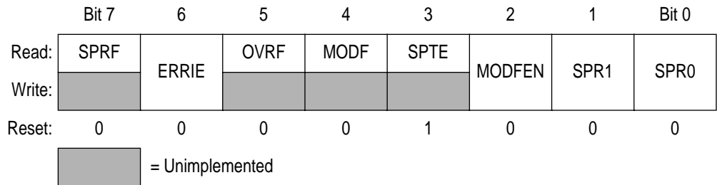
Figure 16-14. SPI Status and Control Register (SPSCR)
