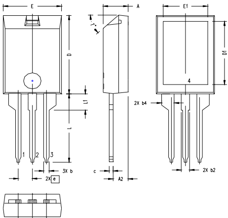
ISOPLUS220 Outline
