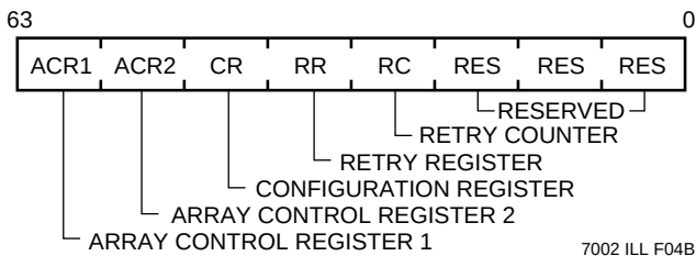
Figure 3. Configuration Registers
