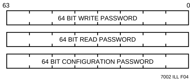
Figure 2. Password Registers
