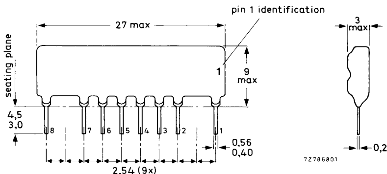
Fig. 2 Encapsulation.
