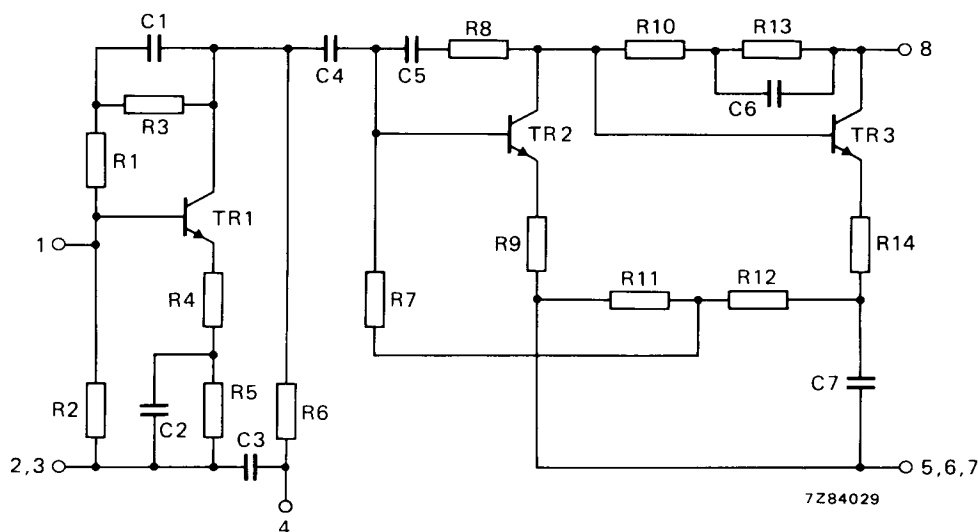
Fig. 1 Circuit diagram.
