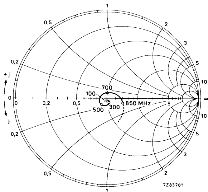
Fig. 6 Output impedance derived from output reflection coefficient s_o , co-ordinates in ohm \times 75 ; typical values.
