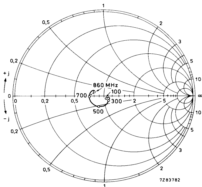
Fig. 5 Input impedance derived from input reflection coefficient s_i , co-ordinates in ohm \times 75 ; typical values.
