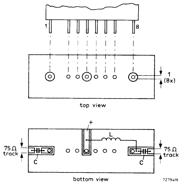
Fig. 3 Printed-circuit board holes and tracks.
