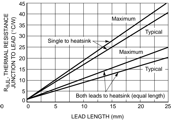
Figure 6. Steady State Thermal Resistance
