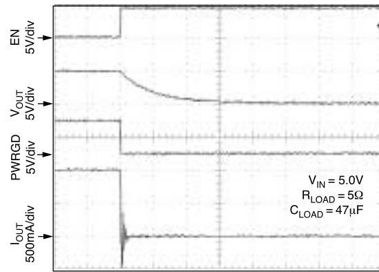
TIME (250μs/div.)
