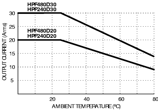
HPF Max. Output Current vs. Temp.
