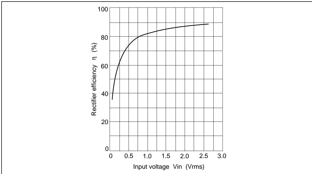
Fig.4 Rectifier efficiency Vs. Input voltage
