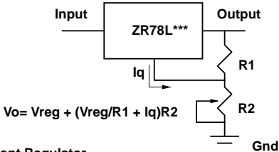
Current Regulator
