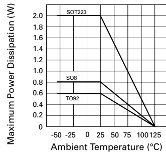
Power dissipation Derating
