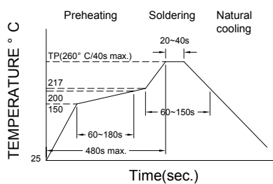
Figure 1. Re-flow Soldering
