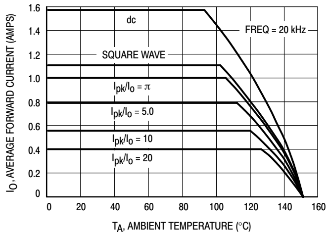
Figure 20. Current Derating
