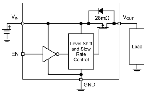
MIC94044 (1ms soft-start)
